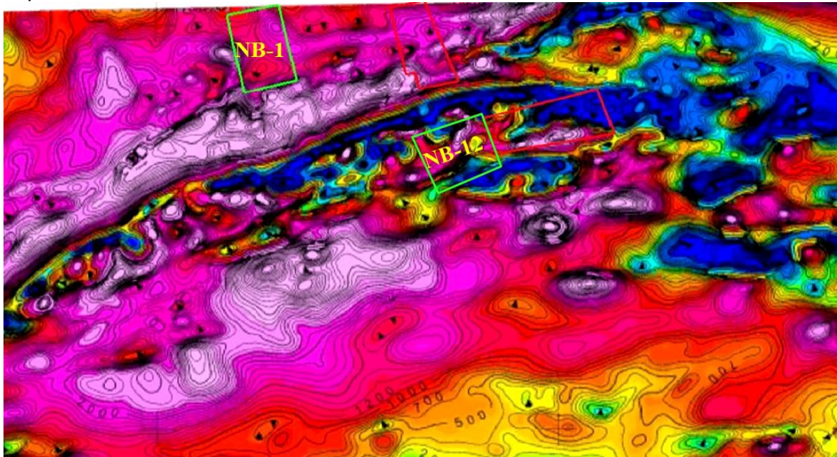
NB-12 Block shown on Aeromag map.
