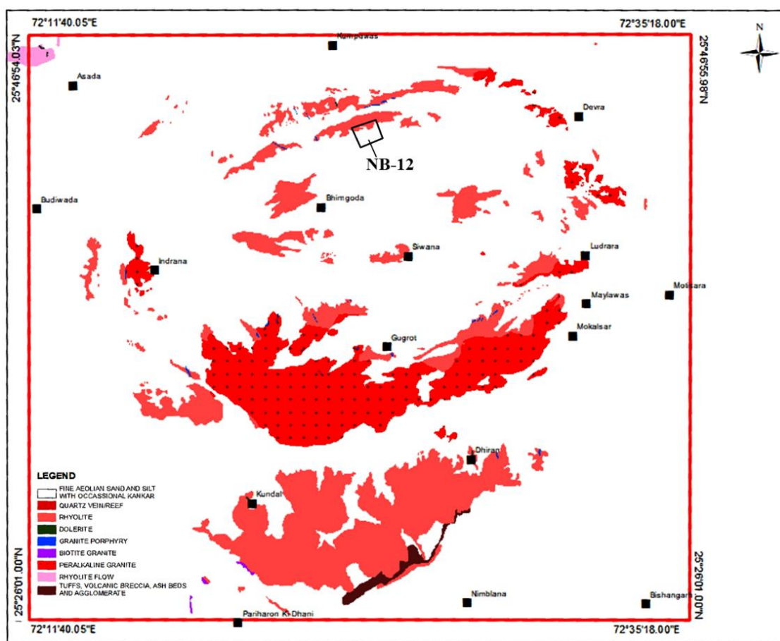
NB-12 block shown on the Geological map of Siwana Ring Complex
