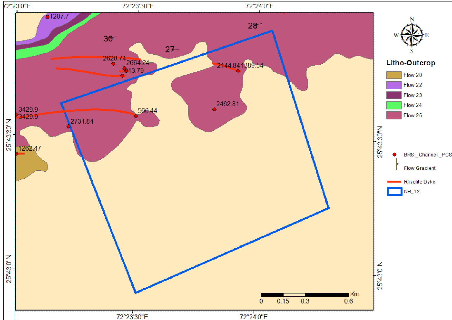
LSM map of NB12 block (Lal and Ghosh, GSI 2023)
